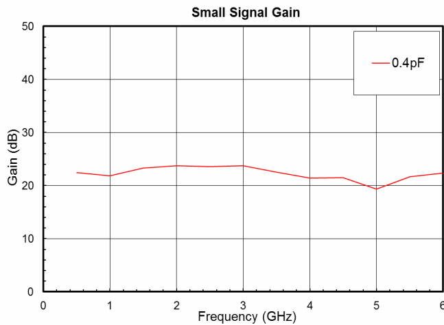
a) Gain under 10%pulse duty cycle
