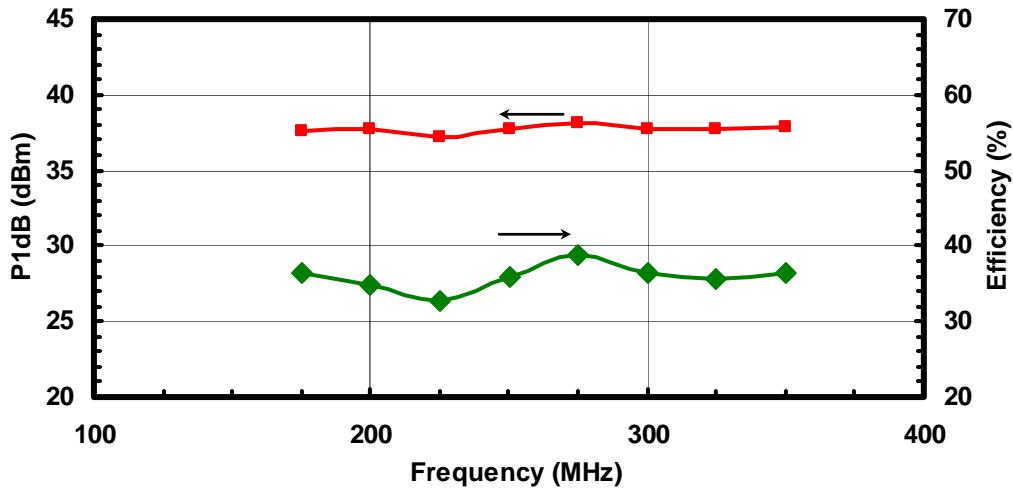
Figure 2a: P_{1dB} and Efficiency vs. Frequency. (Class AB, V_{dd}= +8V , I_{dq}=1.5A , T_a=25^{\circ}C )
